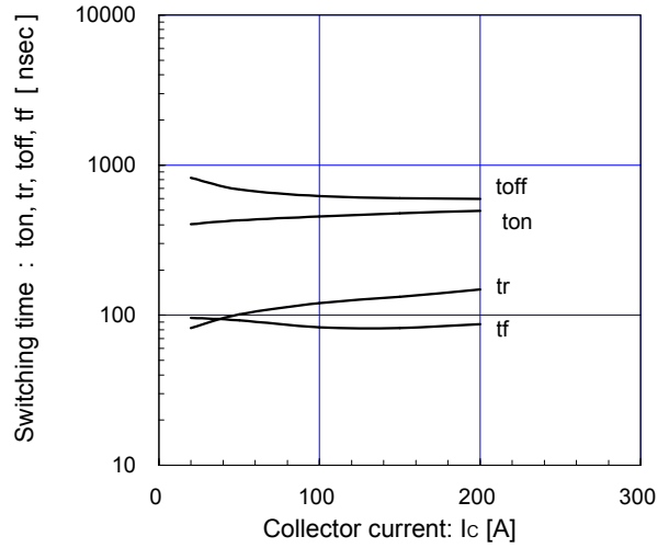
[ Inverter ]
