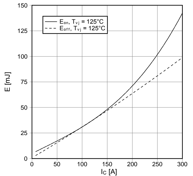
Schaltverluste IGBT-Wechselr. (typisch) switching losses IGBT-inverter (typical) E_{on} = f(I_c) , E_{off} = f(I_c) V_{GE} = \pm 15\text{ V} , R_{Gon} = 9,1\ \Omega , R_{Goff} = 9,1\ \Omega , V_{CE} = 900\text{ V}
