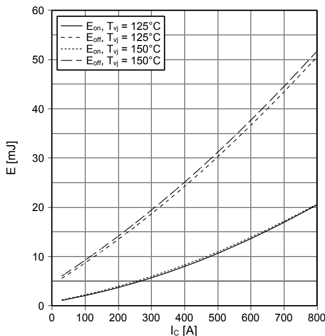
Schaltverluste IGBT-Brems-Chopper switching losses IGBT-brake-chopper E_{on} = f(I_C) , E_{off} = f(I_C) V_{GE} = \pm 15\text{ V} , R_{Gon} = 1.6\ \Omega , R_{Goff} = 1.6\ \Omega , V_{CE} = 300\text{ V}
