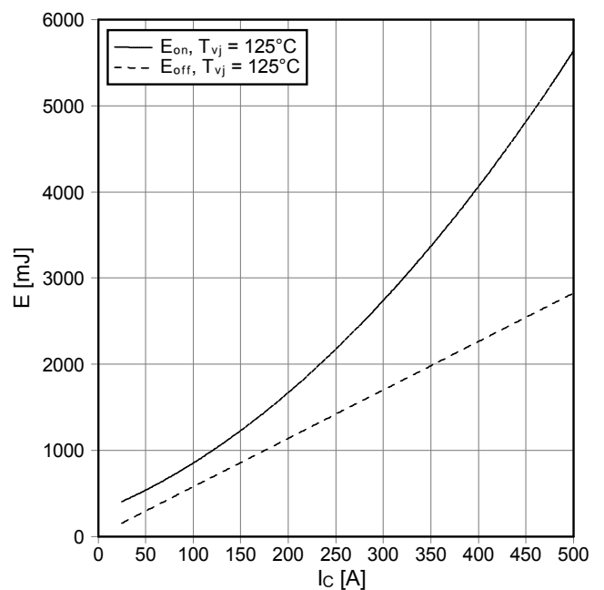
Schaltverluste IGBT-Wechselr. (typisch) switching losses IGBT-inverter (typical) E_{on} = f(I_C), E_{off} = f(I_C) V_{GE} = \pm 15\text{ V}, R_{Gon} = 3\ \Omega, R_{Goff} = 20.4\ \Omega, V_{CE} = 3600\text{ V}
