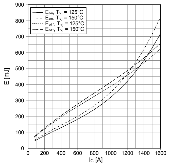
Schaltverluste IGBT-Wechselr. (typisch) switching losses IGBT-inverter (typical) E_{on} = f(I_c), E_{off} = f(I_c) V_{GE} = \pm 15\text{ V}, R_{Gon} = 0.39\ \Omega, R_{Goff} = 2.2\ \Omega, V_{CE} = 900\text{ V}
