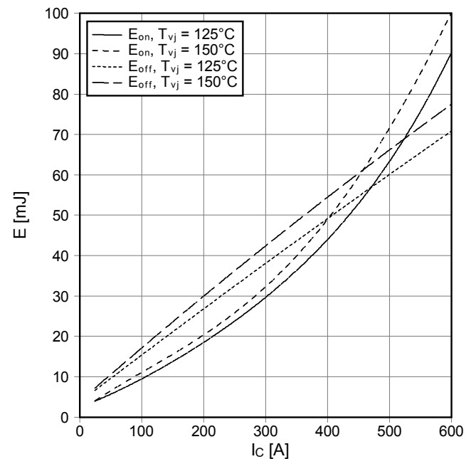
Schaltverluste IGBT-Wechselr. (typisch) switching losses IGBT-inverter (typical) E_{on} = f(I_c), E_{off} = f(I_c) V_{GE} = \pm 15\text{ V}, R_{Gon} = 0.75\ \Omega, R_{Goff} = 0.75\ \Omega, V_{CE} = 600\text{ V}
