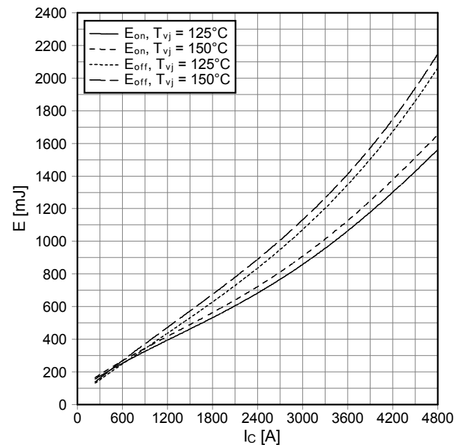
Schaltverluste IGBT-Wechselr. (typisch) switching losses IGBT-inverter (typical) E_{on} = f(I_c), E_{off} = f(I_c) V_{GE} = \pm 15\text{ V}, R_{Gon} = 0.5\ \Omega, R_{Goff} = 0.5\ \Omega, V_{CE} = 900\text{ V}
