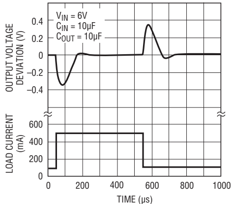
LT1763-5 Transient Response C_{\text{BYP}} = 0
