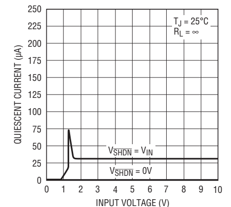
LT1763-1.5 Quiescent Current
