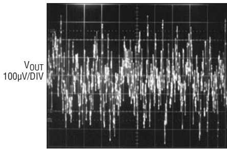
C_{\text{OUT}} = 10\mu\text{F} I_{\text{L}} = 500\text{mA}
