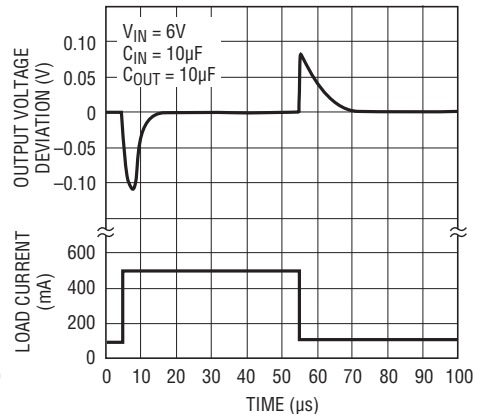
LT1763-5 Transient Response C_{\text{BYP}} = 0.01\mu\text{F}
