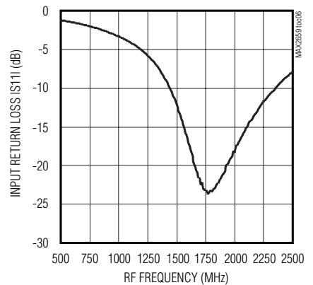
INPUT RETURN LOSS vs. RF FREQUENCY
