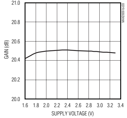
GAIN vs. SUPPLY VOLTAGE
