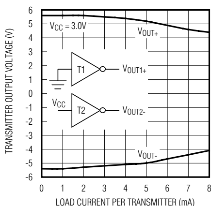
Figure 2. Transmitter Output Voltage vs. Load Current per Transmitter
