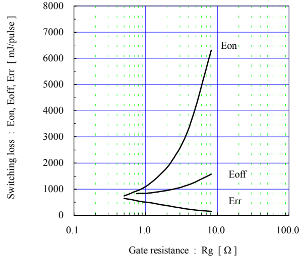
Switching loss vs. Gate resistance (typ.) V_{cc}=900V, I_c=2400A, V_{GE}=\pm 15V, T_j=125^\circ C
