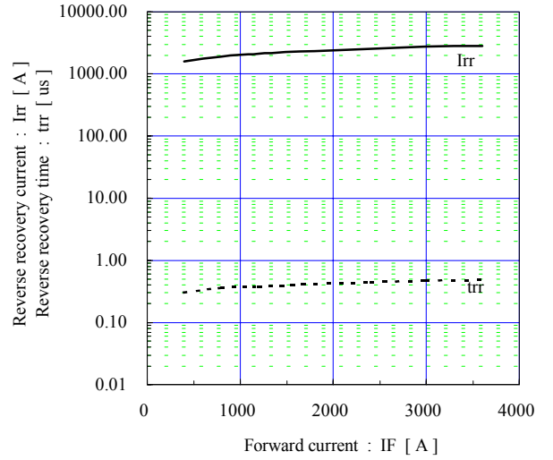
Reverse recovery characteristics (typ.) Vcc=900V, VGE=±15V, Rg=0.2Ω, Tj=125°C
