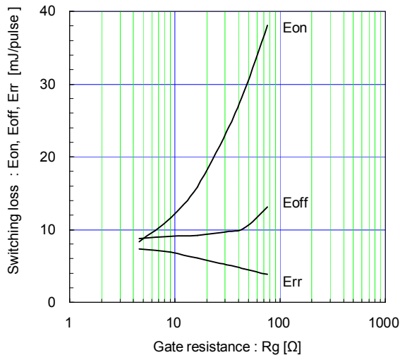
Switching loss vs. Gate resistance (typ.) Vcc=600V, Ic=100A, VGE=±15V, Tj= 125°C
