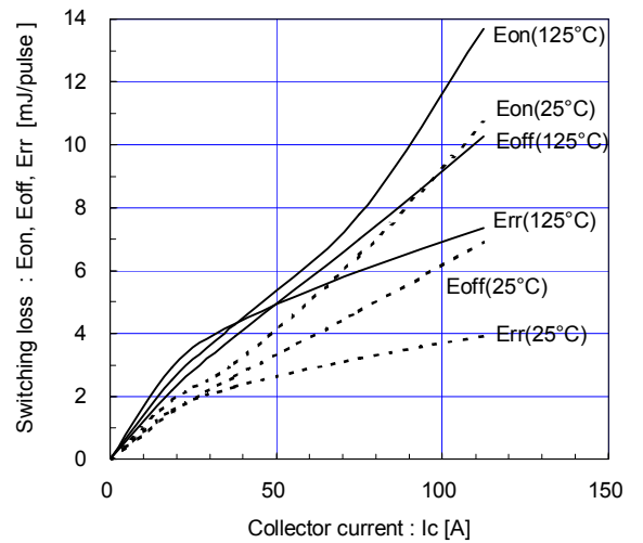
Switching loss vs. Collector current (typ.) Vcc=600V, VGE=±15V, Rg=9.1Ω
