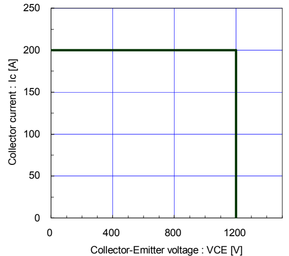
Reverse bias safe operating area (max.) +VGE=15V, -VGE ≤ 15V, Rg ≥ 9.1Ω, Tj ≤ 125°C
