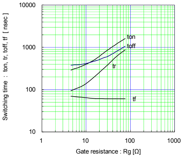
Switching time vs. Gate resistance (typ.) Vcc=600V, Ic=100A, VGE=±15V, Tj= 25°C
