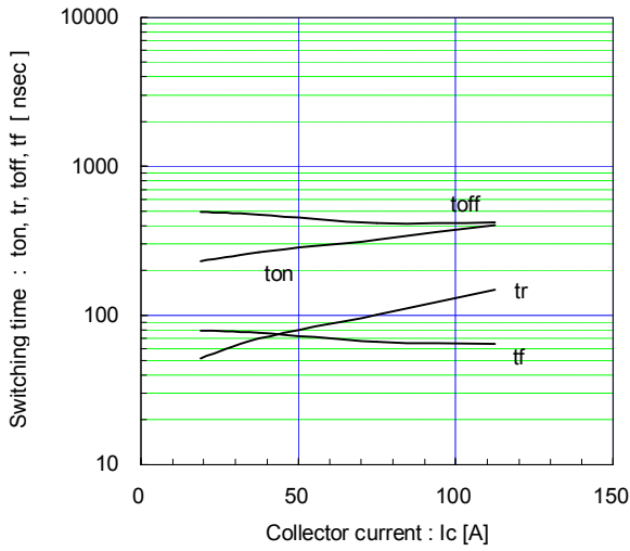
Switching time vs. Collector current (typ.) Vcc=600V, VGE=±15V, Rg=9.1Ω, Tj= 25°C
