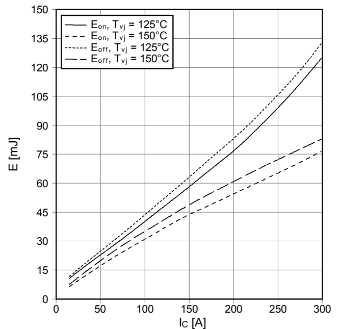
Schaltverluste IGBT-Wechselr. (typisch) switching losses IGBT-inverter (typical) E_{on} = f(I_c), E_{off} = f(I_c) V_{GE} = \pm 15\text{ V}, R_{Gon} = 4.8\ \Omega, R_{Goff} = 4.8\ \Omega, V_{CE} = 900\text{ V}
