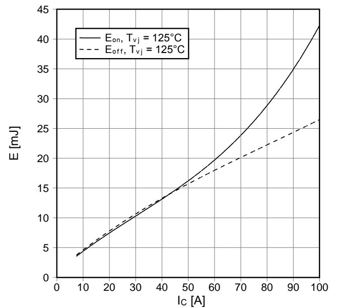
Schaltverluste IGBT-Wechselr. (typisch) switching losses IGBT-inverter (typical) E_{on} = f(I_C), E_{off} = f(I_C) V_{GE} = \pm 15\text{ V}, R_{Gon} = 8\ \Omega, R_{Goff} = 8\ \Omega, V_{CE} = 900\text{ V}
