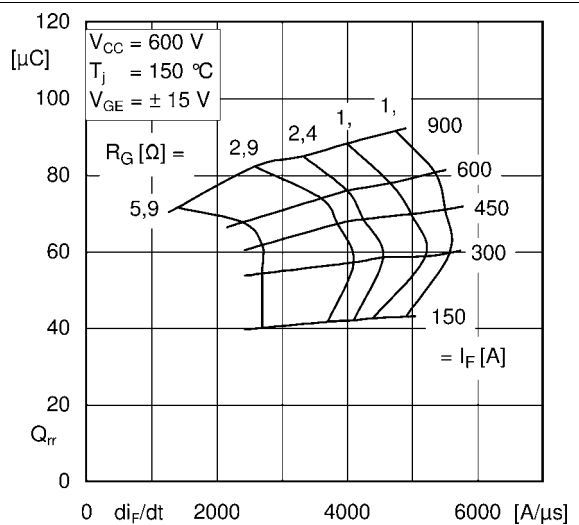
Fig. 12: Typ. CAL diode recovery charge
