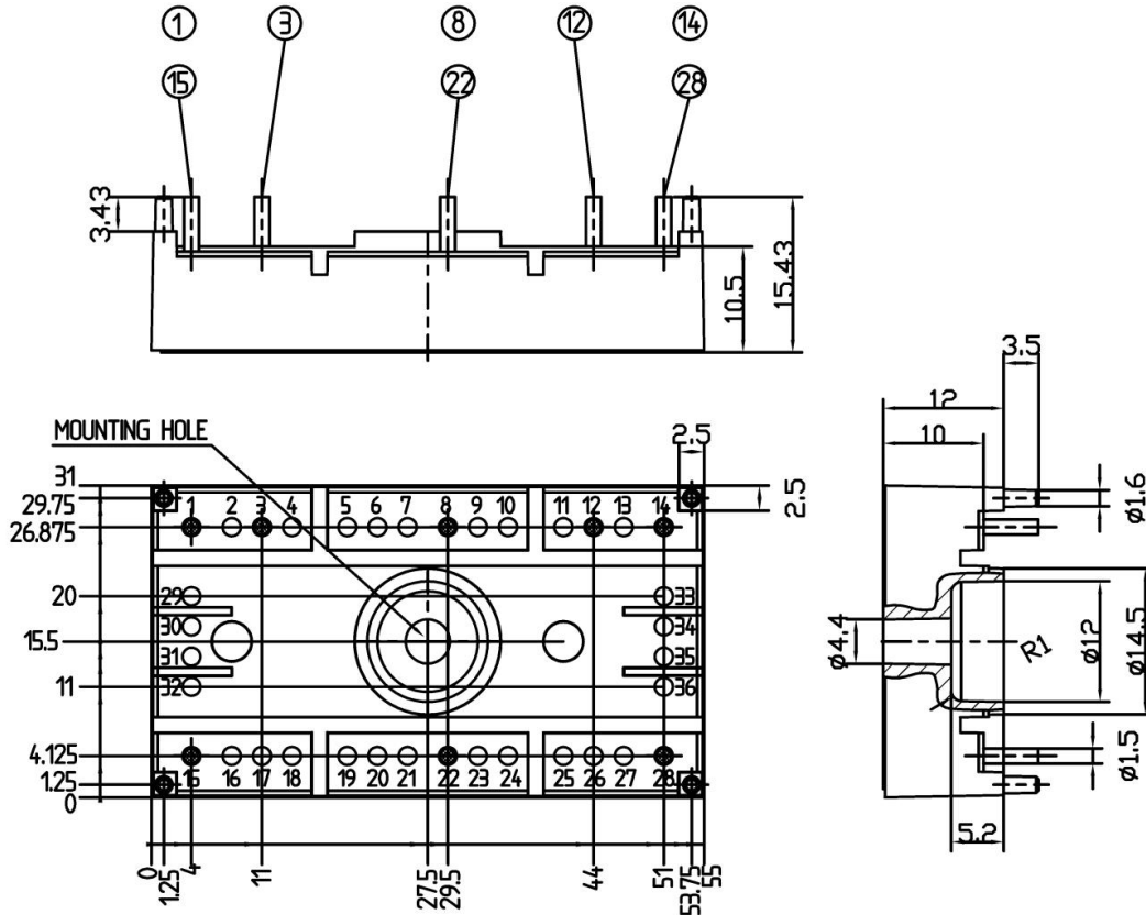
Case T20 (Suggested hole diameter, in the PCB, for solder pins and plastic mounting pins: 2mm)
