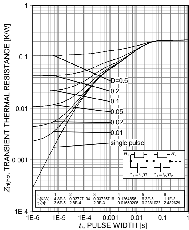
Figure 21. IGBT transient thermal resistance ( D = t_p/T )
