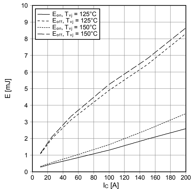
Schaltverluste IGBT-Wechselr. (typisch) switching losses IGBT-inverter (typical) E_{on} = f(I_c), E_{off} = f(I_c) V_{GE} = \pm 15\text{ V}, R_{Gon} = 3.9\ \Omega, R_{Goff} = 3.9\ \Omega, V_{CE} = 300\text{ V}
