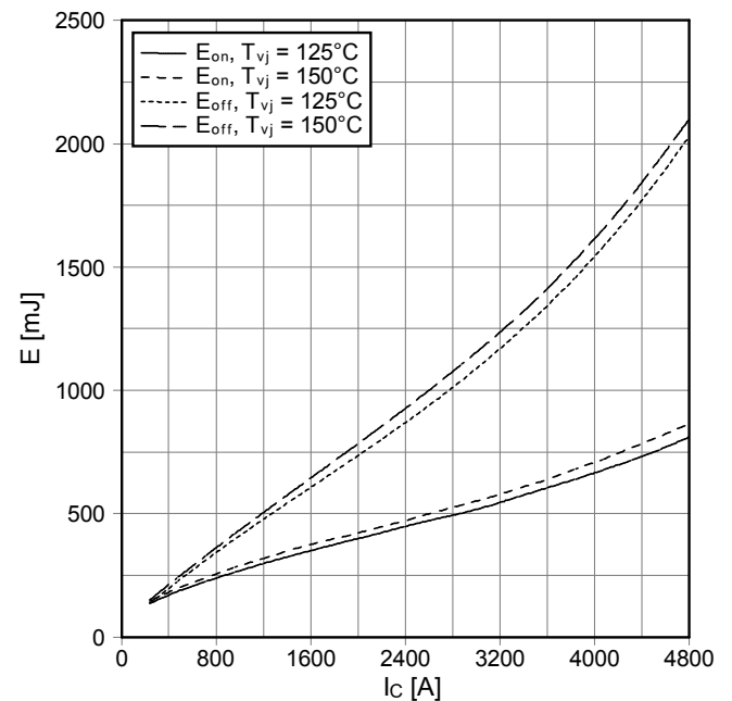
Schaltverluste IGBT-Wechselr. (typisch) switching losses IGBT-inverter (typical) E_{on} = f(I_c) , E_{off} = f(I_c) V_{GE} = \pm 15\text{ V} , R_{Gon} = 0.6\ \Omega , R_{Goff} = 0.4\ \Omega , V_{CE} = 900\text{ V}
