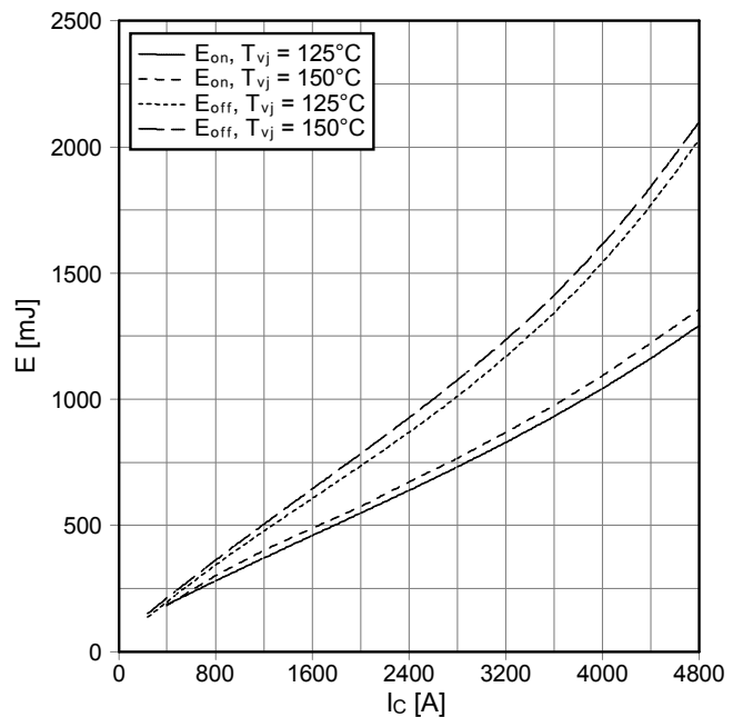
Schaltverluste IGBT-Wechselr. (typisch) switching losses IGBT-inverter (typical) E_{on} = f(I_c) , E_{off} = f(I_c) V_{GE} = \pm 15\text{ V} , R_{Gon} = 0.8\ \Omega , R_{Goff} = 0.4\ \Omega , V_{CE} = 900\text{ V}
