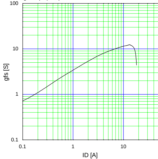
Typical Transconductance
