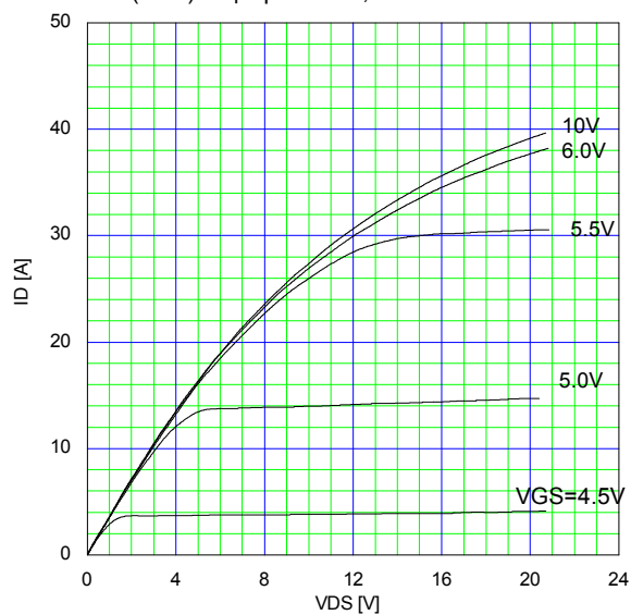
Typical Output Characteristics I_D = f(V_{DS}) : 80 μs pulse test, T_{ch} = 25\text{ °C}
