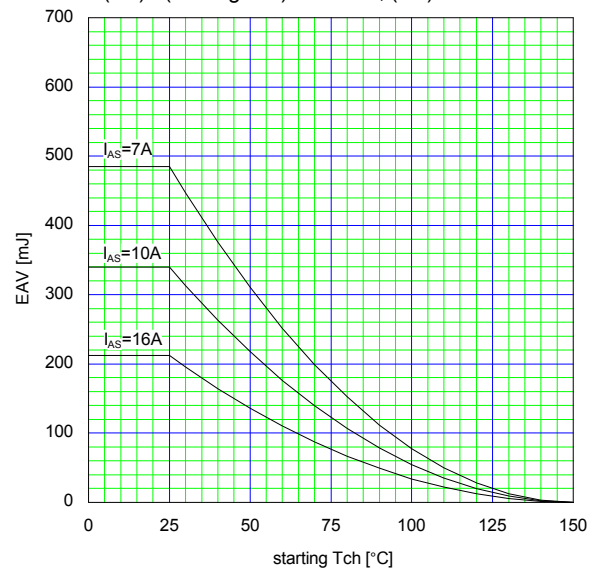
Maximum Avalanche Energy vs. starting Tch E(AV)=f(\text{starting Tch}):V_{cc}=50V, I(AV)\leq 16A
