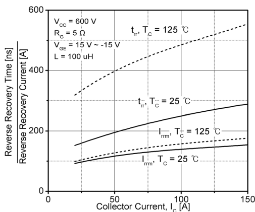
Fig 11. Typical Recovery Characteristics of Diode
